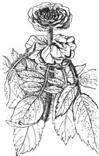
FIG. 150. — Proliferous Rose. (From Masters, Vegetable Teratology .)
